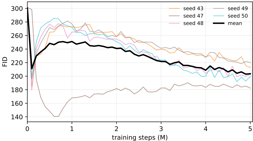
CIFAR-10 d=260
